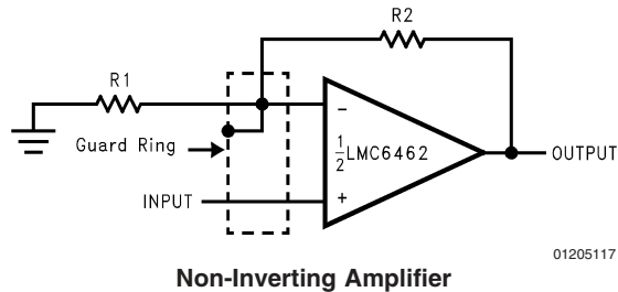
Non-Inverting Amplifier
