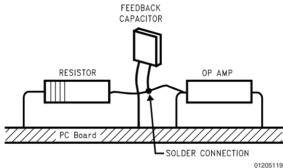
FIGURE 13. Air Wiring
